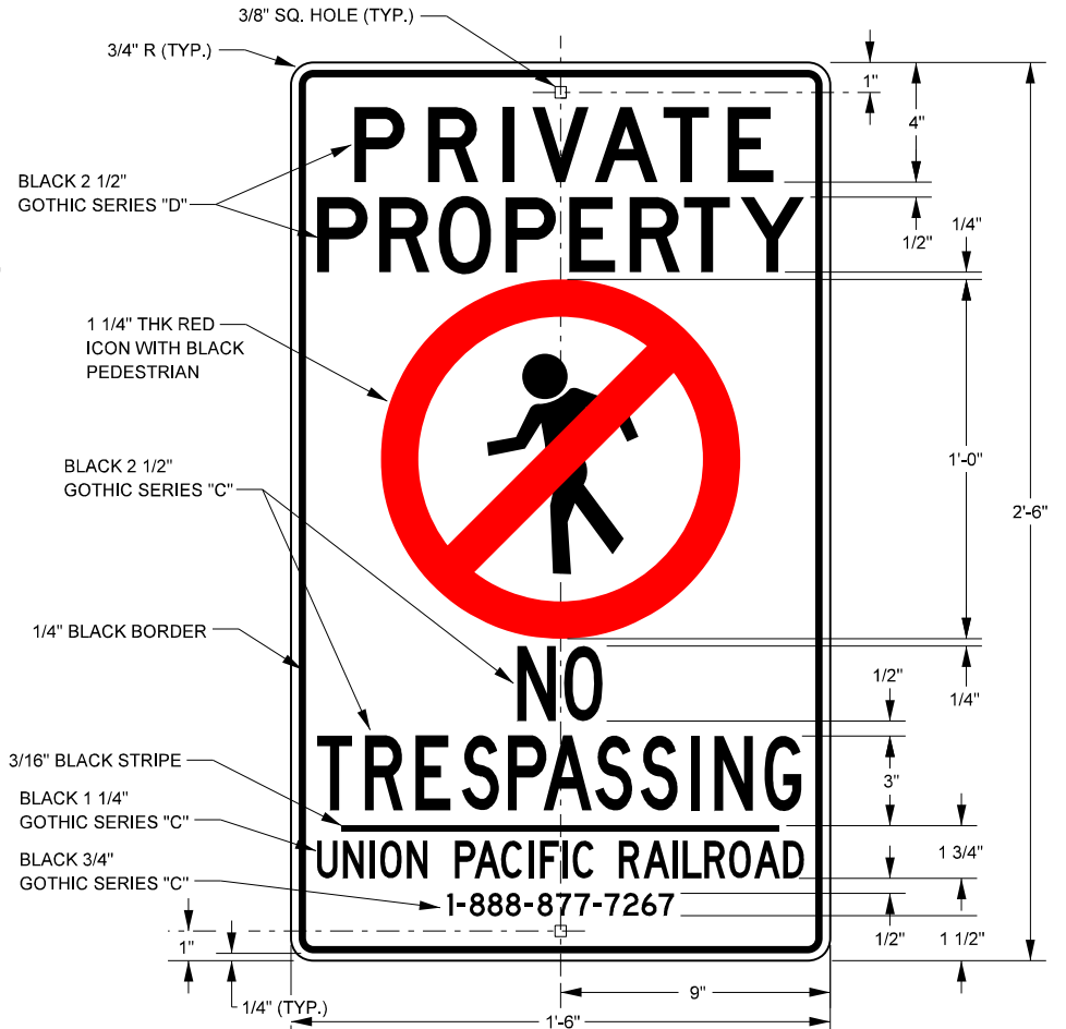
ALUMINUM SIGN ITEM NO. 393-3651 COMPOSITE SIGN ITEM NO. 393-3653 (COMPOSITE SIGN FOR USE IN HIGH THEFT AREAS)
